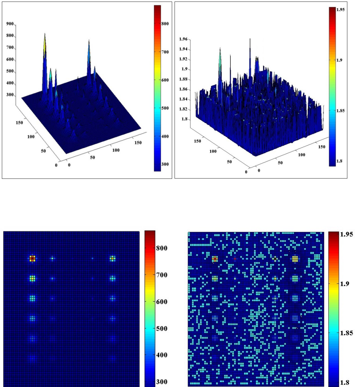
Figure 4.10 Amplitudegram [°C] on left and Phasegram [rad] on right as 3D on top and 2D on bottom respectively, generated by MATLAB (Appendix B.1)
