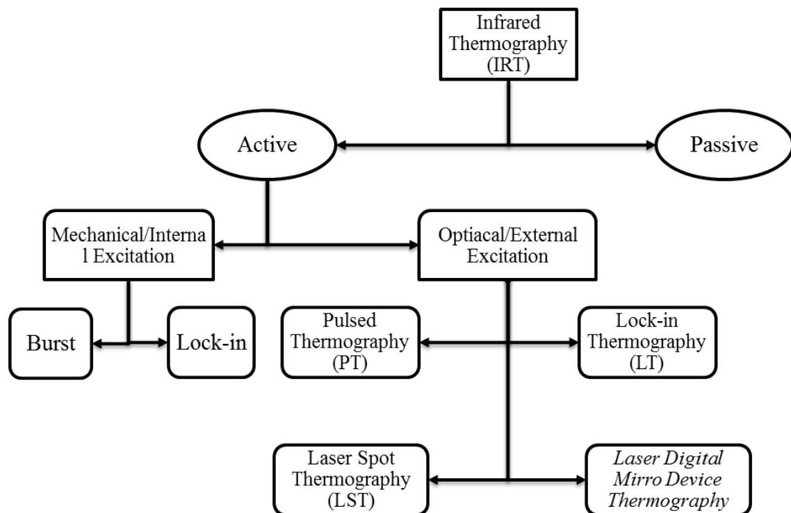
Figure 2.3 Infrared thermography classifications
