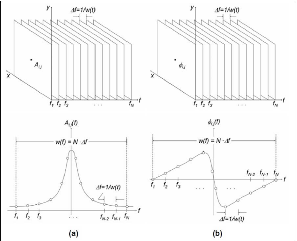
Figure 4.4 (a) Amplitgram (Amplitude gram); and (b) phasegram sequences; on top, and their corresponding profiles on the frequency spectra for a non-defective pixel on coordinates (i, j); on bottom [36]
