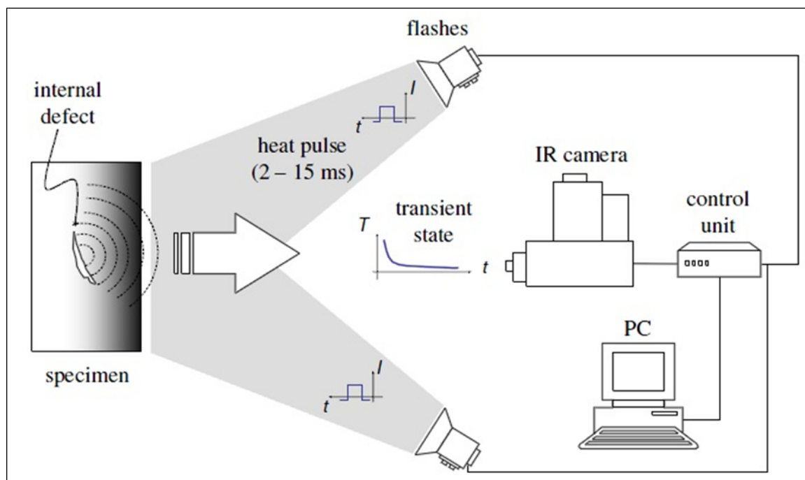
Figure 3.1 Equipment configurations for Pulse Thermography Flash or Transient [34]
